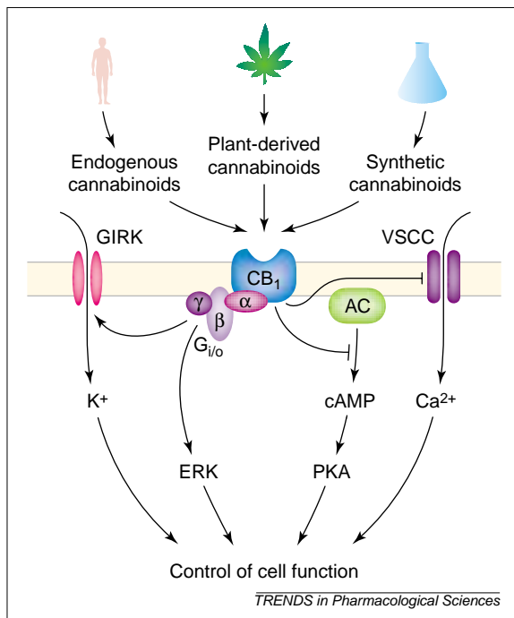
Fig. 1. G-protein-coupled signalling pathways activated by the cannabinoid CB 1 receptor. Endogenous, plant-derived and synthetic cannabinoids produce most of their effects by binding to the CB 1 receptor. This G i/o -protein-coupled receptor signals inhibition of the adenylyl cyclase (AC)–protein-kinase-A (PKA) pathway and activation of the extracellular signal-regulated kinase (ERK) cascade. In addition, the CB 1 receptor modulates ion channels, inducing, for example, inhibition of N- and P/Q-type voltage-sensitive Ca 2+ channels (VSCCs) and activation of G-protein-activated inwardly rectifying K + channels (GIRKs). All these events participate in the control of cell function by cannabinoids.
